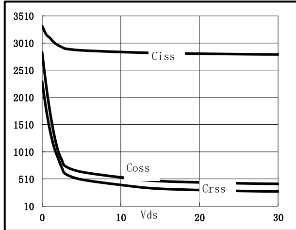
Fig.8 Capacitance Characteristics
