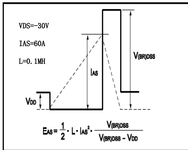
Fig.12 Avalanche Waveform
