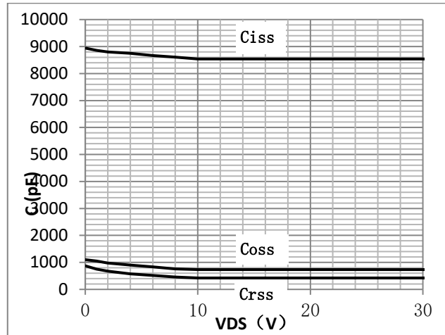
Fig.2 Capacitance Characteristics
