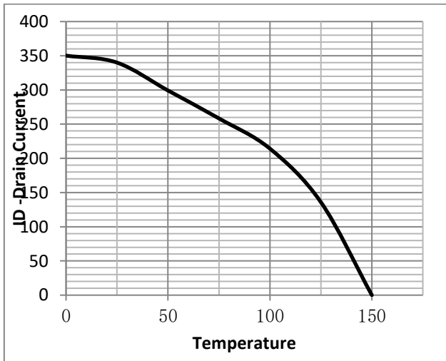
Fig.12 ID-Junction Temperature
