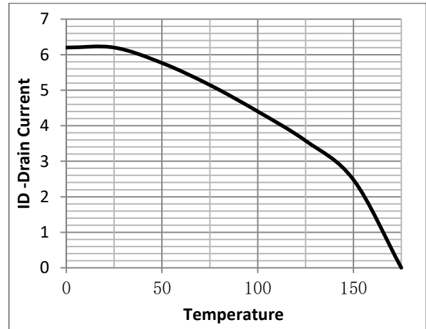
Fig.10 Drain Current V.S Junction Temperature
