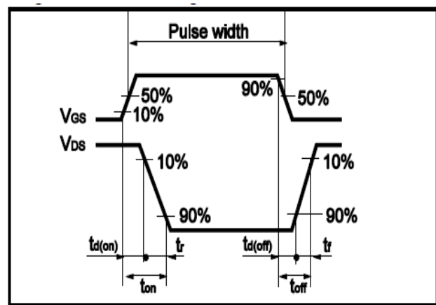
Fig.16 Resistive Switching Test Waveform
