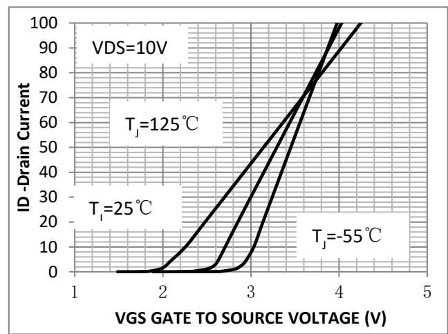
Figure 10. Transfer Characteristics
