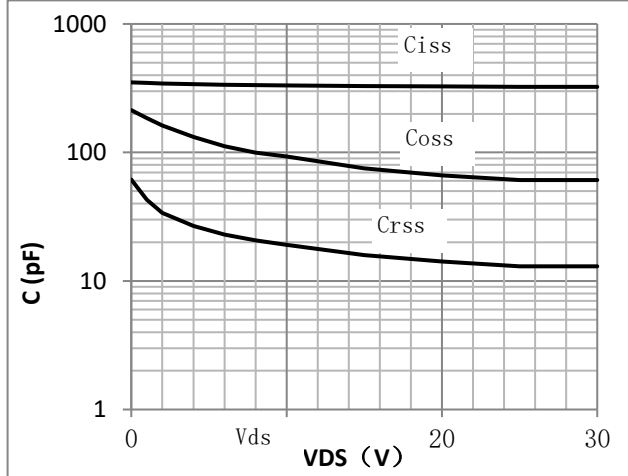
Fig.2 Capacitance Characteristics
