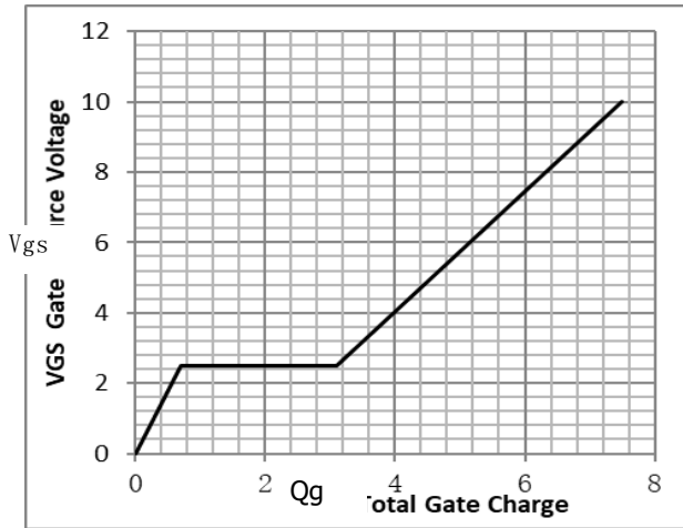
Fig.1 Gate-Charge Characteristics
