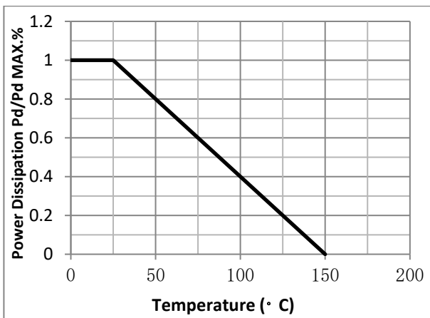
Fig.1 Power Dissipation
