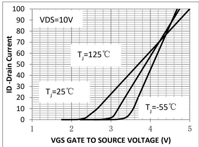
Figure 10. Transfer Characteristics
