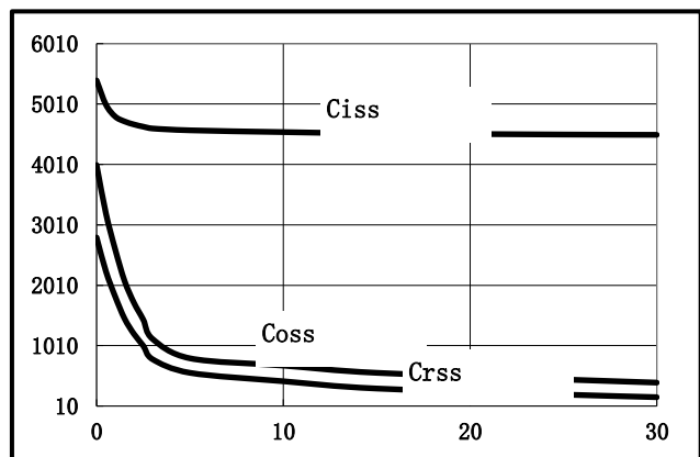
Fig.2 Capacitance Characteristics
