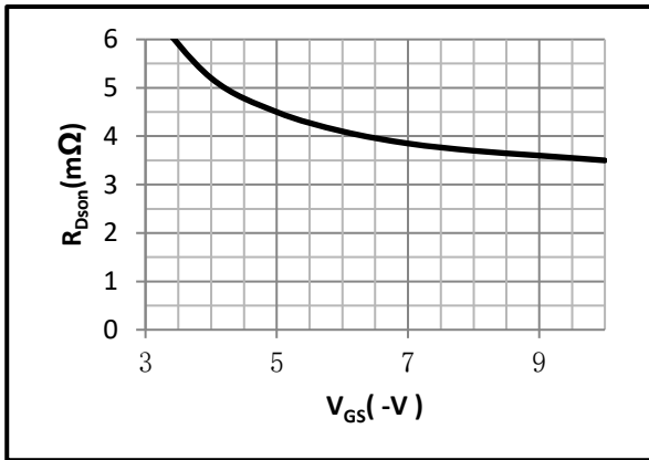
ig.7 On-Resistance VS Gate Source Voltage
