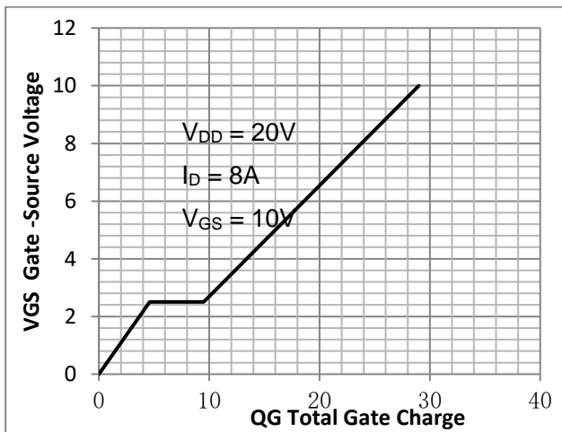
Figure 11. Gate-to-Source and Drain-to-Source Voltage vs. Total Charge
