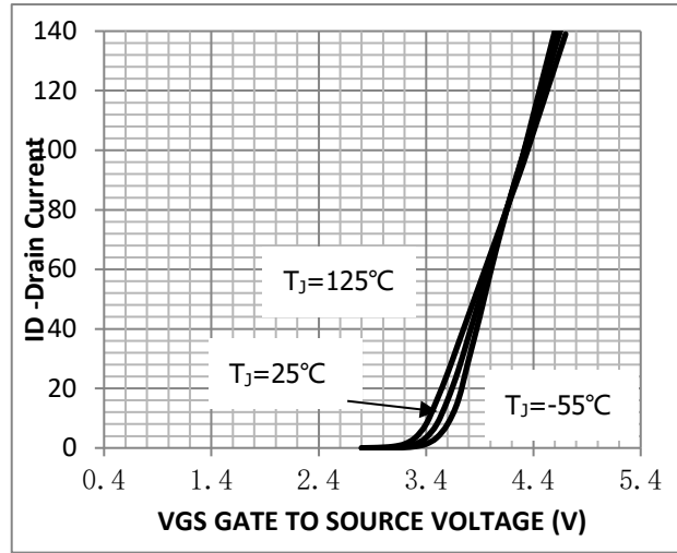
Figure 12. Transfer Characteristics
