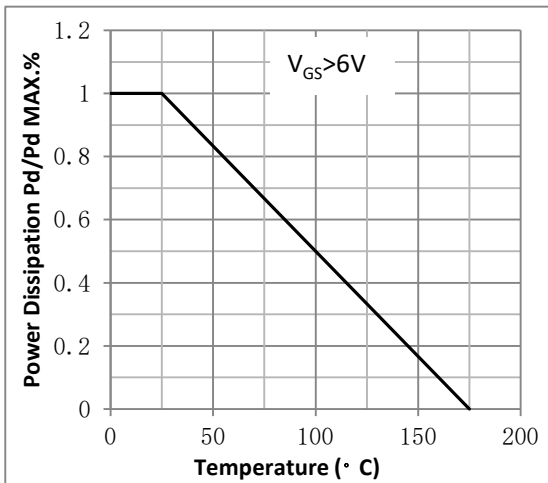
Fig.3 Power Dissipation
