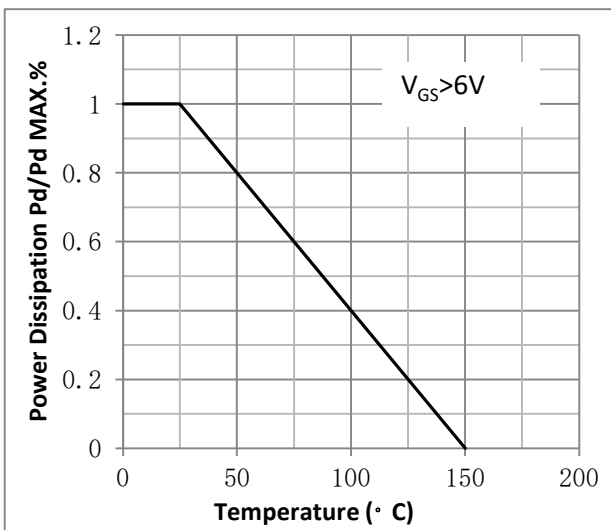
Fig.3 Power Dissipation
